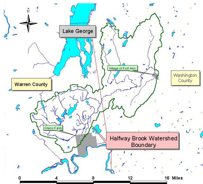
Halfway Brook watershed location map
