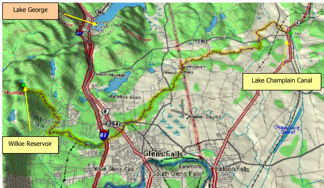
Topography of the Halfway Brook watershed
